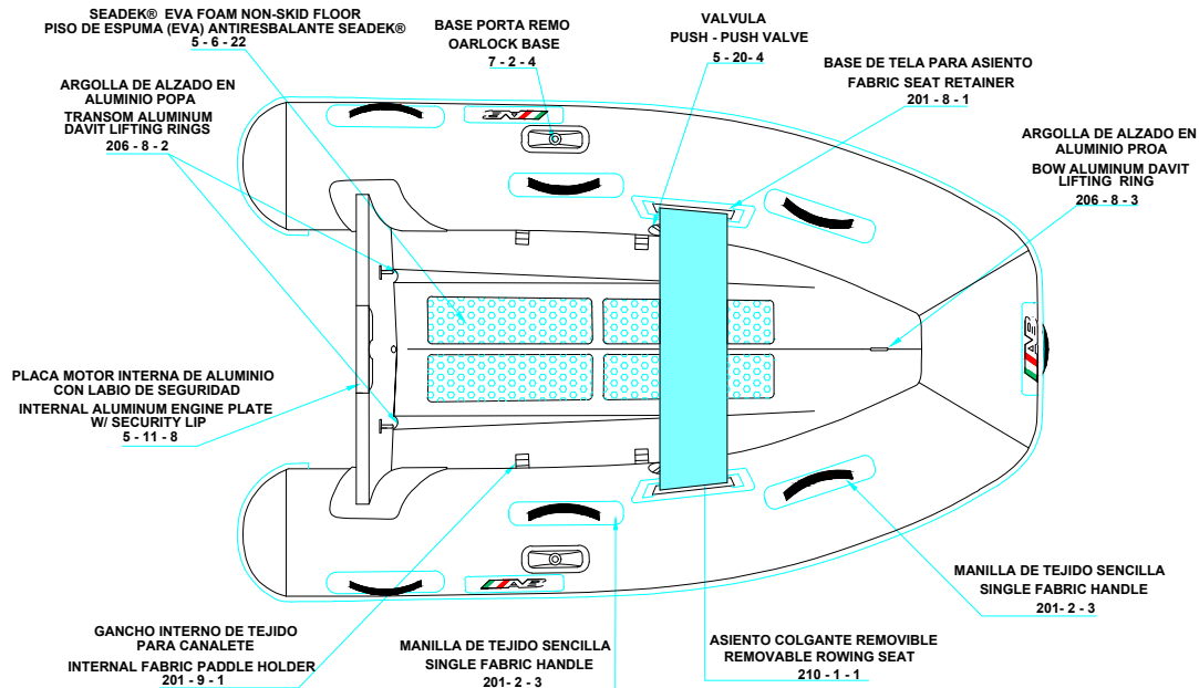
PLANT VIEW VISTA SUPERIOR
