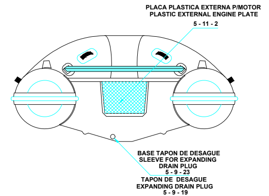
AFT VIEW VISTA TRASERA
