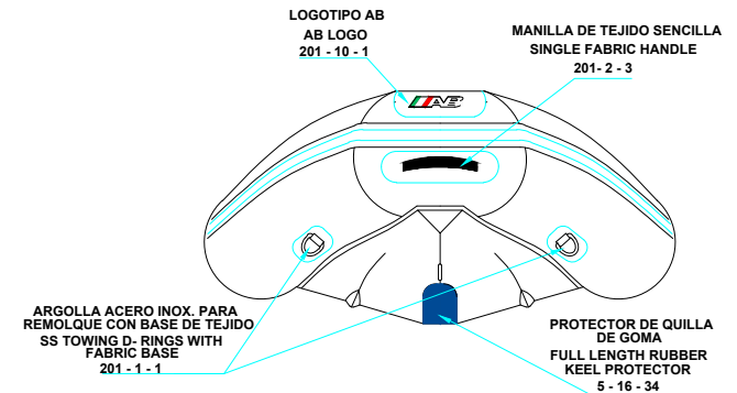
FORE VIEW VISTA FRONTAL
