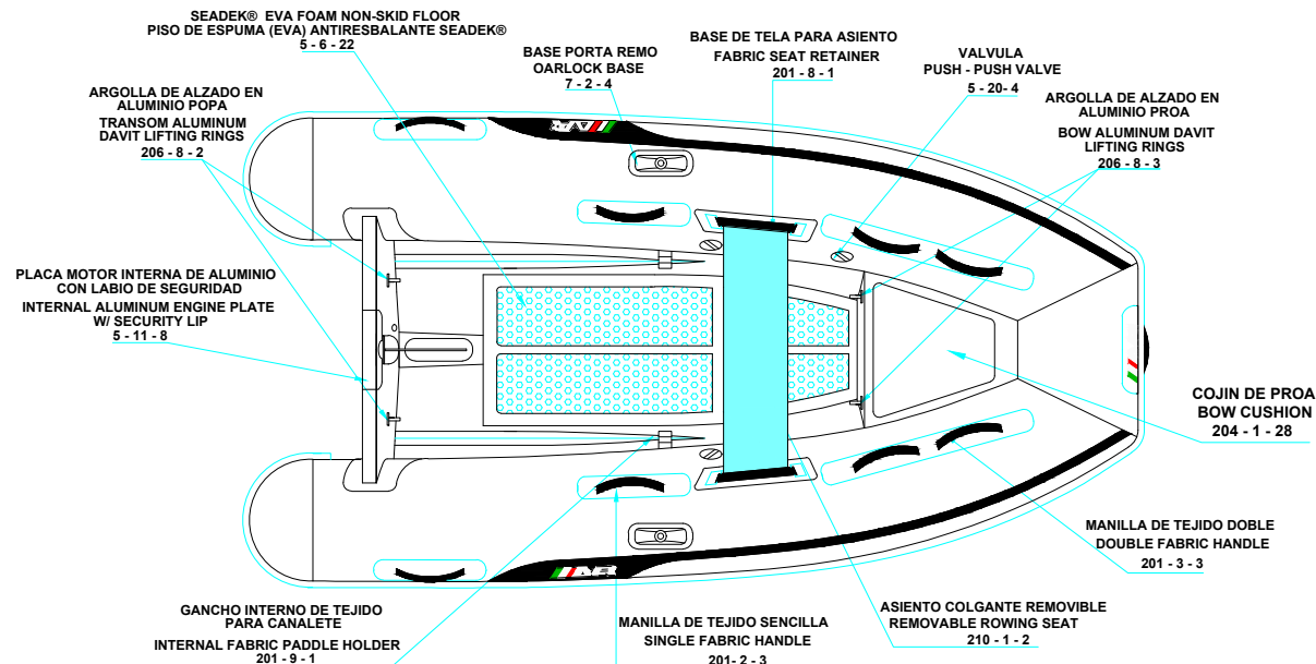
PLANT VIEW VISTA SUPERIOR
