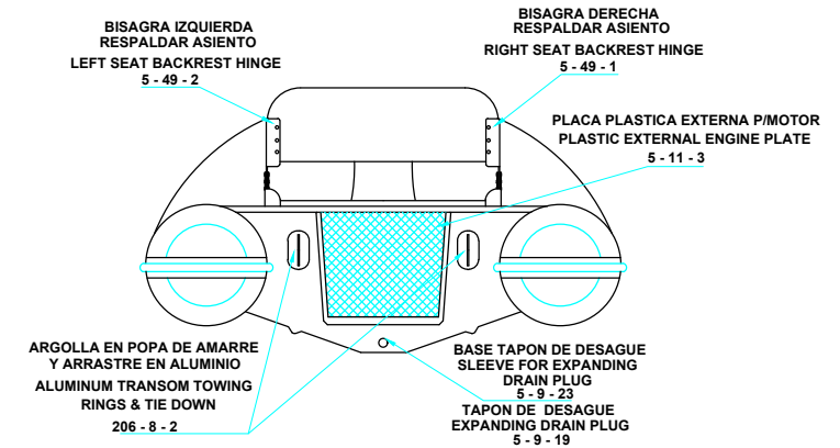
AFT VIEW VISTA TRASERA
