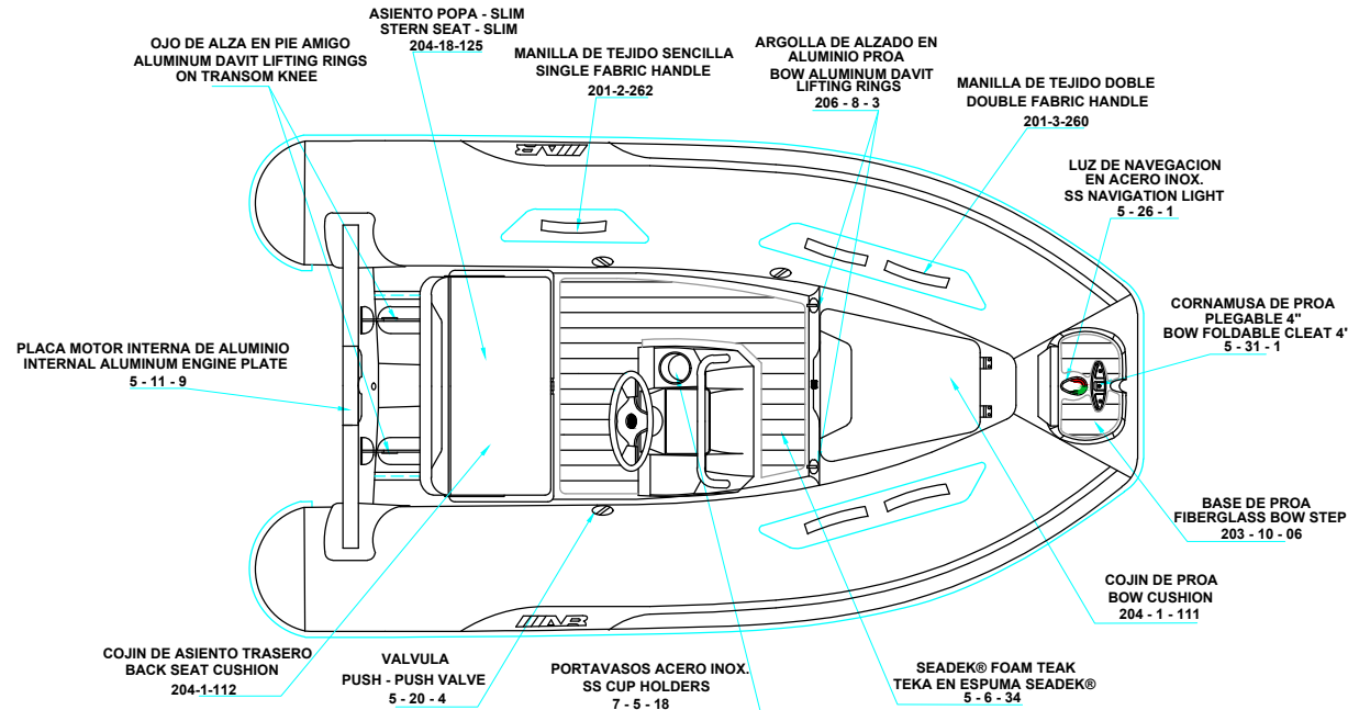
PLANT VIEW VISTA SUPERIOR
