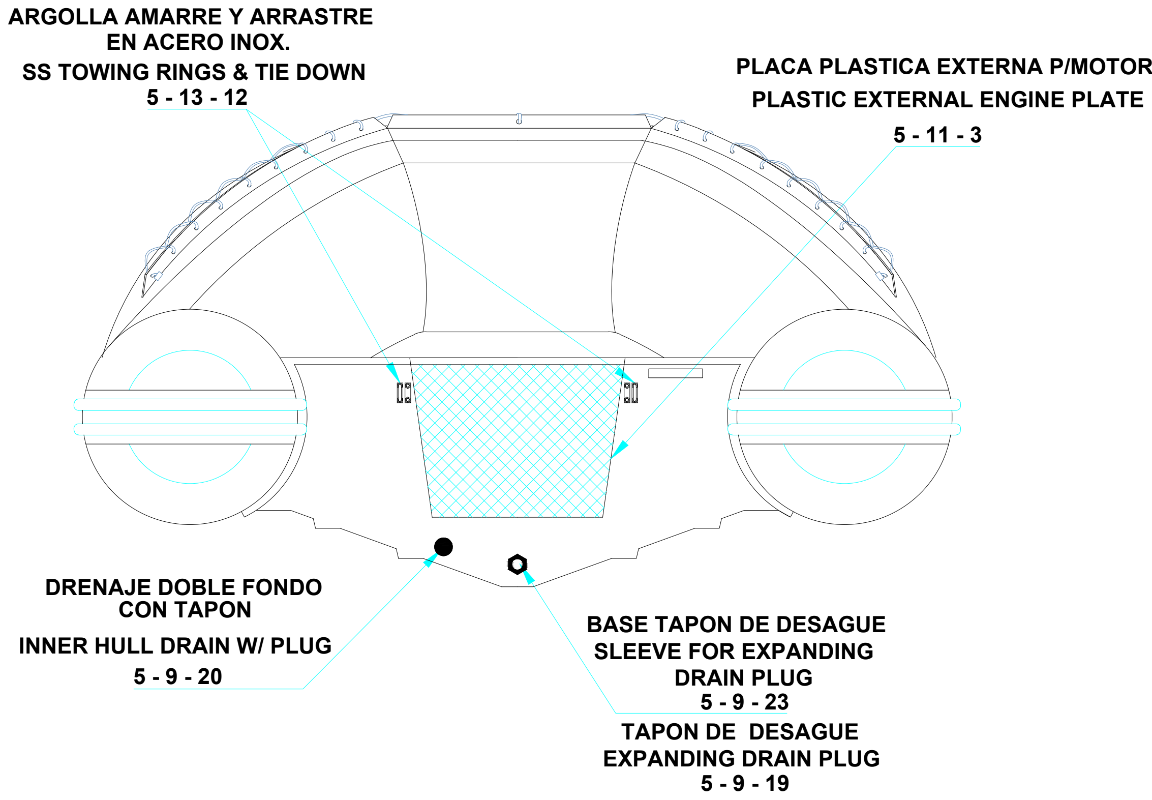
AFT VIEW VISTA TRASERA
