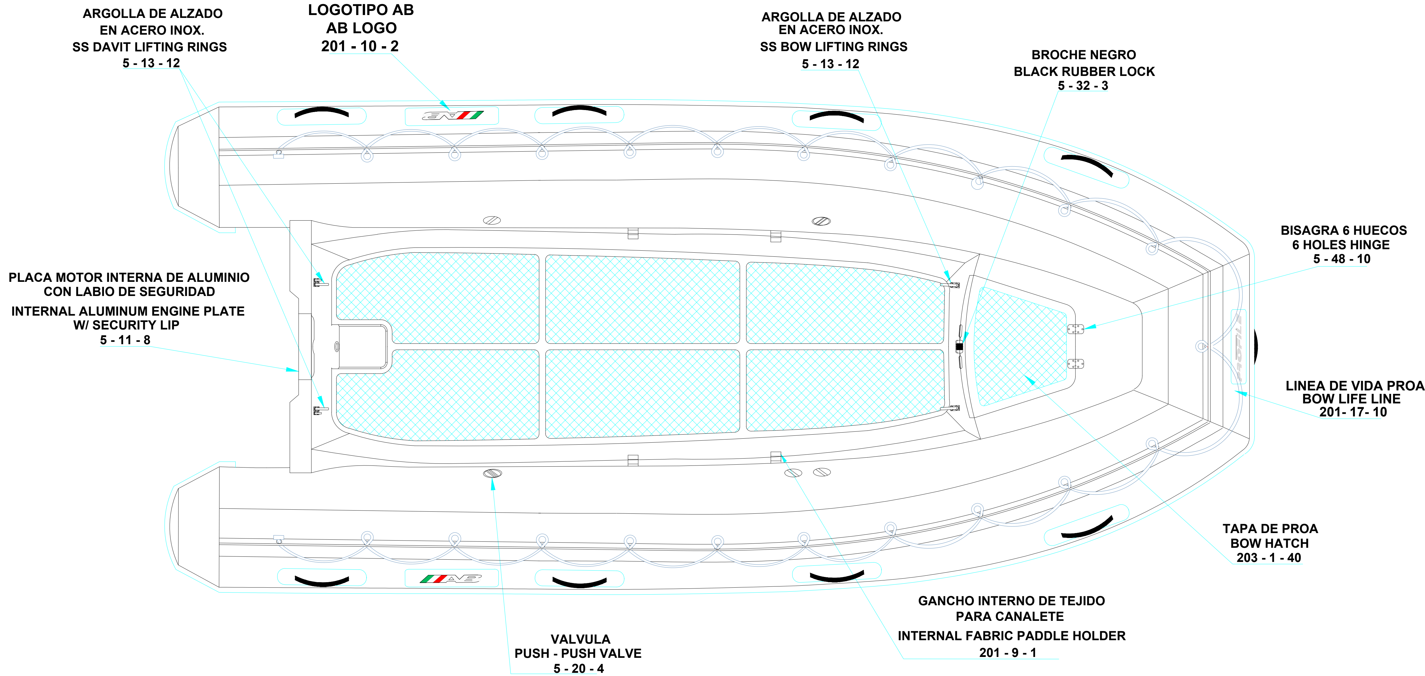
PLANT VIEW VISTA SUPERIOR
