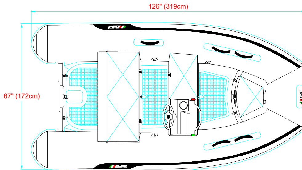
PLANT VIEW VISTA SUPERIOR
