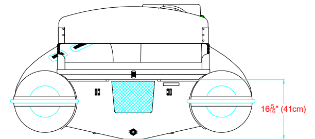
AFT VIEW VISTA TRASERA
