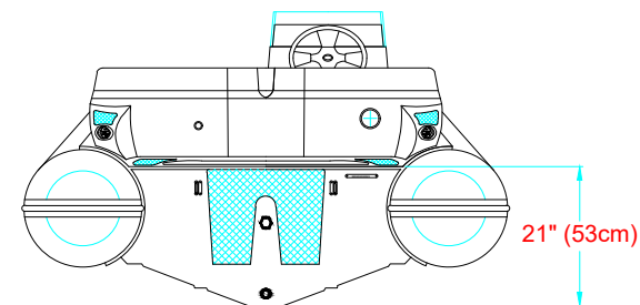
AFT VIEW VISTA TRASERA
