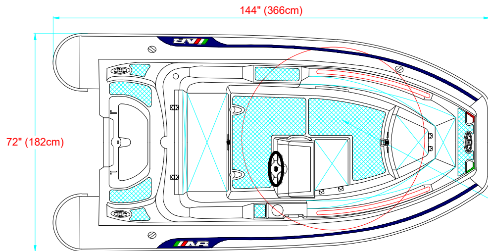
PLANT VIEW VISTA SUPERIOR
