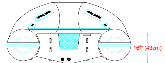
AFT VIEW VISTA TRASERA
