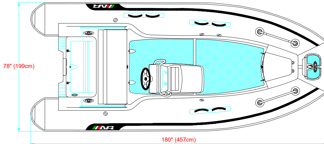
PLANT VIEW VISTA SUPERIOR
