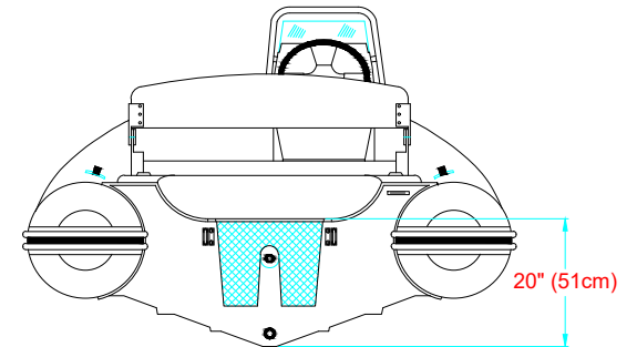
AFT VIEW VISTA TRASERA
