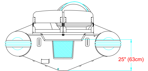
AFT VIEW VISTA TRASERA
