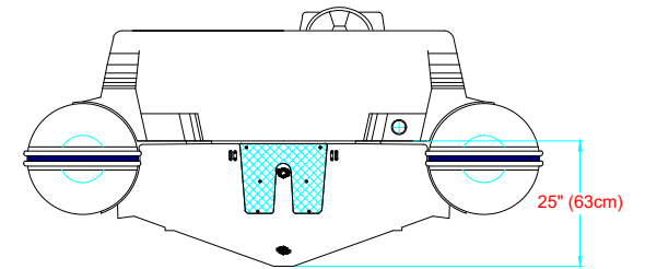
AFT VIEW VISTA FRONTAL
