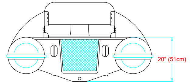
AFT VIEW VISTA TRASERA
