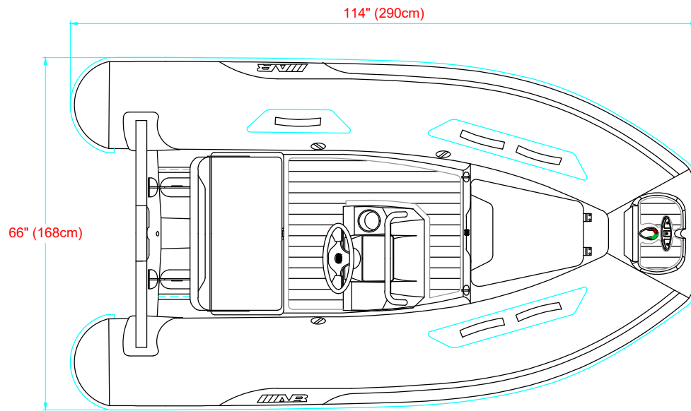
PLANT VIEW VISTA SUPERIOR
