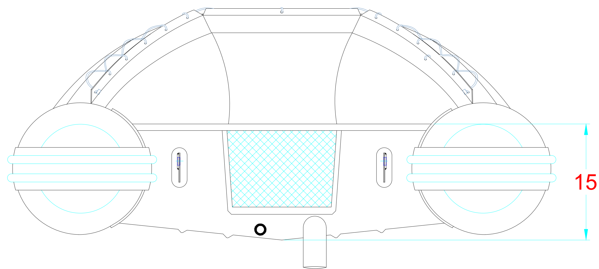
AFT VIEW VISTA TRASERA
