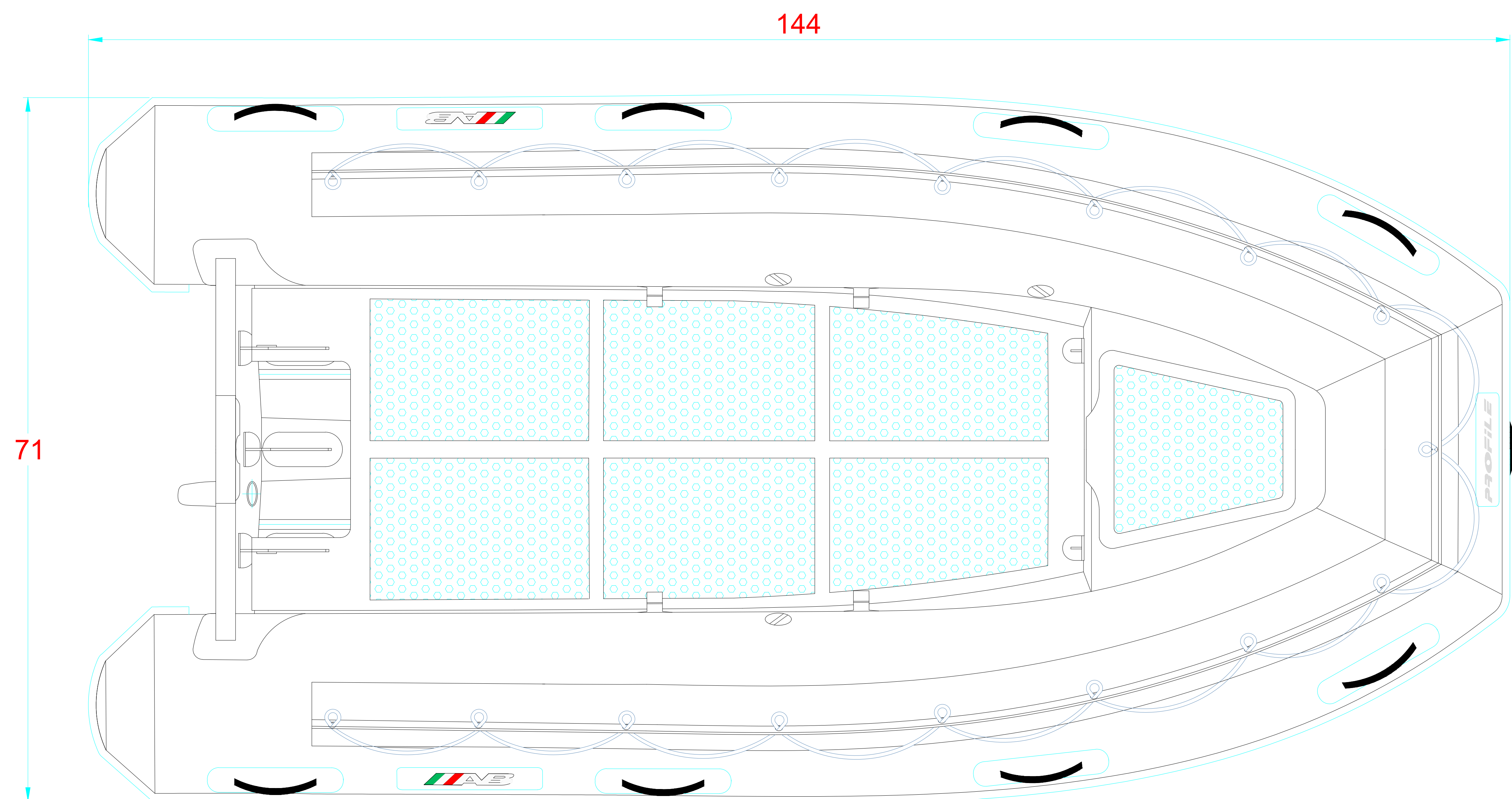
PLANT VIEW VISTA SUPERIOR
