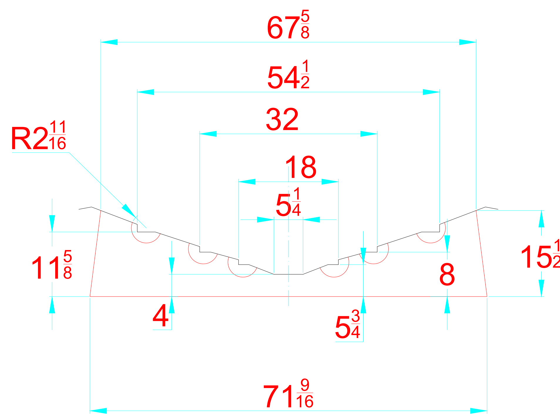
TRANSVERSAL SECTION "A" SECCION TRANSVERSAL "A"
