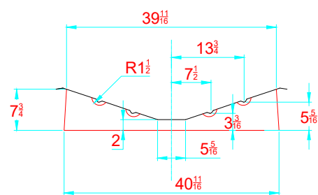
TRANSVERSAL SECTION "A" SECCION TRANSVERSAL "A"
