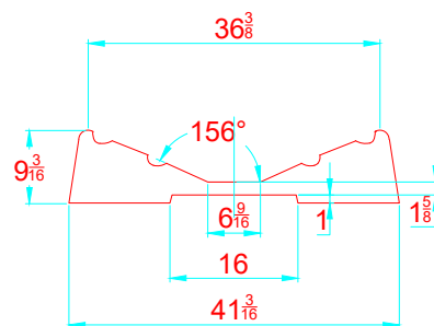
TRANSVERSAL SECTION "A" SECCION TRANSVERSAL "A"
