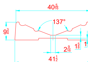
TRANSVERSAL SECTION "A" SECCION TRANSVERSAL "A"
