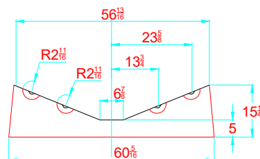
TRANSVERSAL SECTION "A" SECCION TRANSVERSAL "A"
