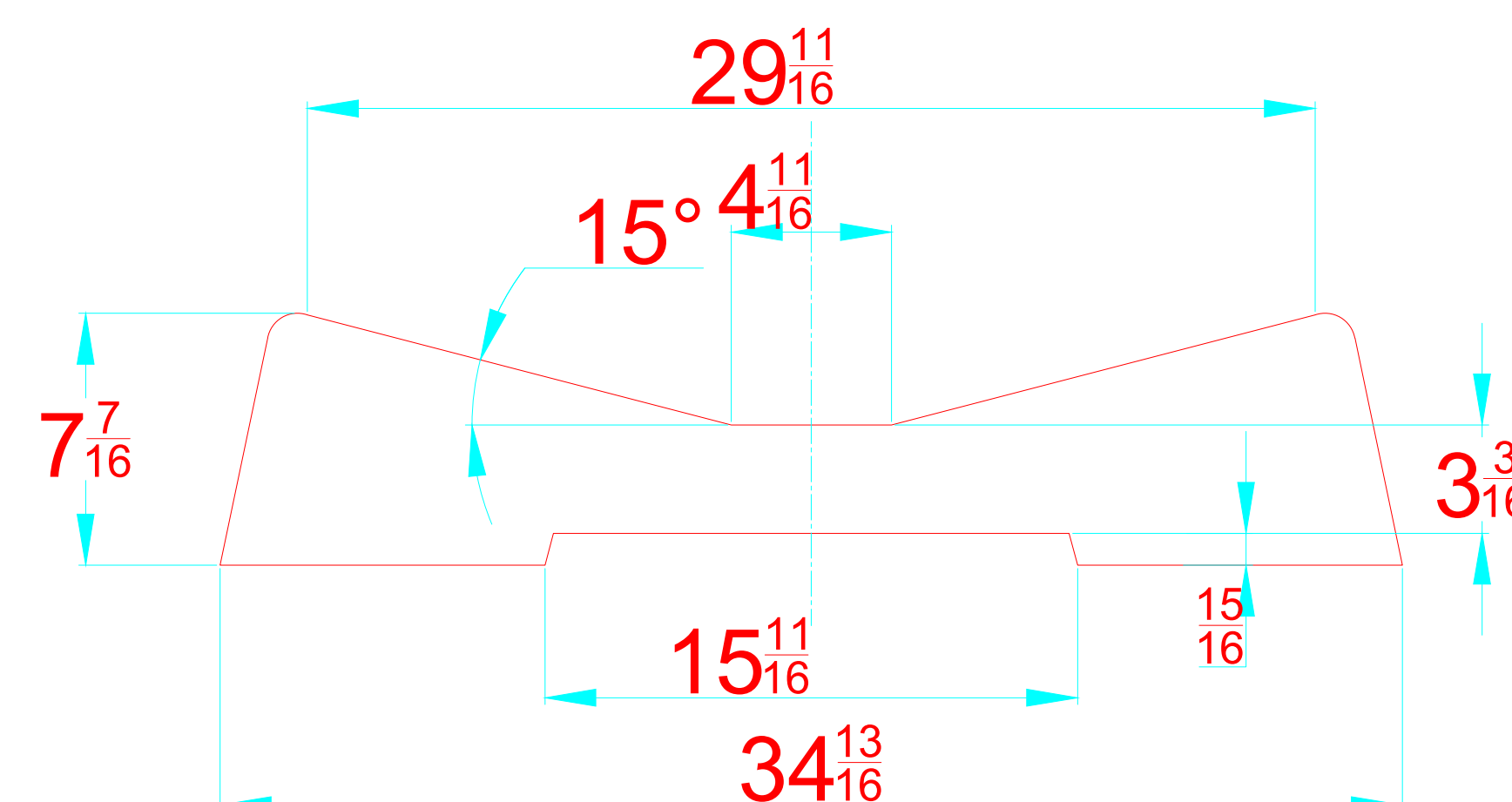
TRANSVERSAL SECTION "A" SECCION TRANSVERSAL "A"
