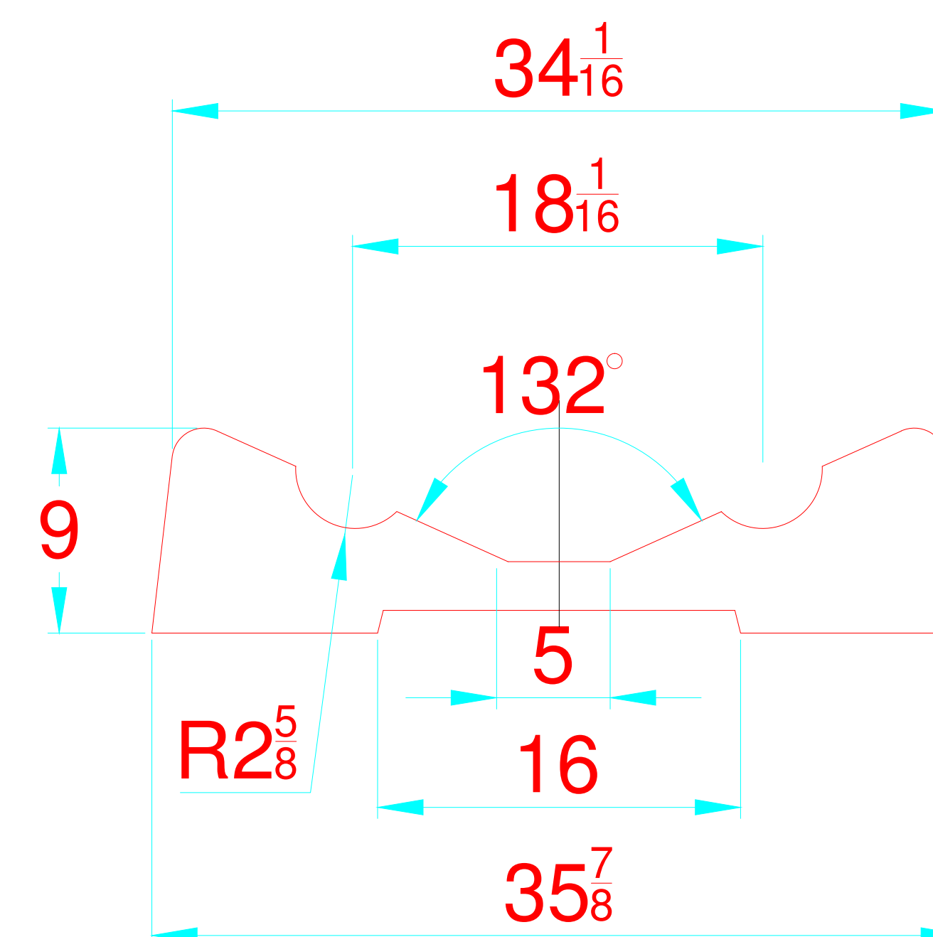
TRANSVERSAL SECTION "A" SECCION TRANSVERSAL "A"
