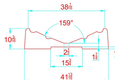
TRANSVERSAL SECTION "A" SECCION TRANSVERSAL "A"
