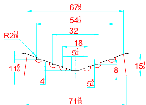
TRANSVERSAL SECTION "A" SECCION TRANSVERSAL "A"
