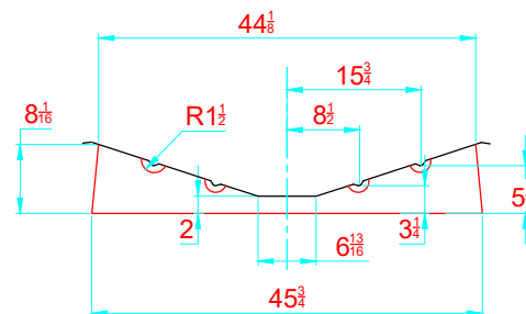
TRANSVERSAL SECTION "A" SECCION TRANSVERSAL "A"
