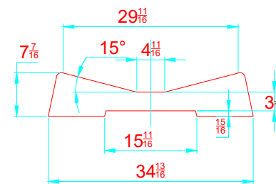
TRANSVERSAL SECTION "A" SECCION TRANSVERSAL "A"
