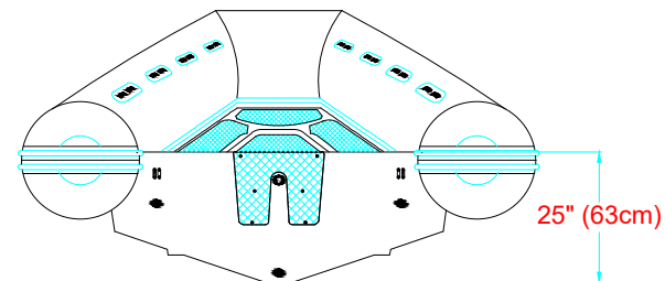
AFT VIEW VISTA TRASERA
