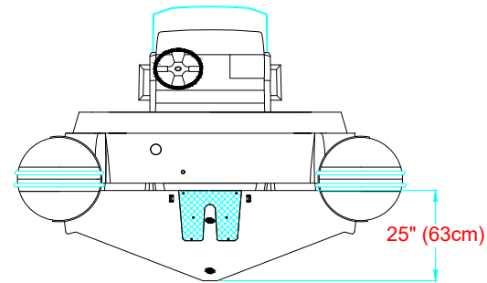
AFT VIEW VISTA TRASERA
