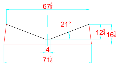
TRANSVERSAL SECTION "A" SECCION TRANSVERSAL "A"
