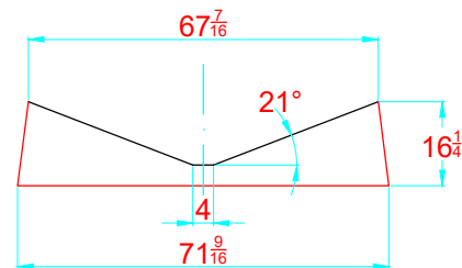
TRANSVERSAL SECTION "A" SECCION TRANSVERSAL "A"
