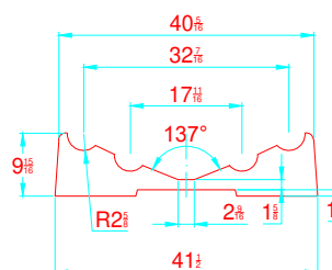
TRANSVERSAL SECTION "A" SECCION TRANSVERSAL "A"
