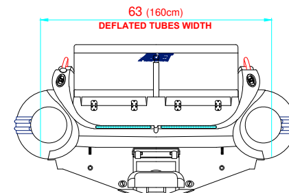
AFT VIEW VISTA TRASERA
