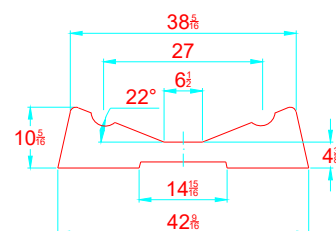
TRANSVERSAL SECTION "A" SECCION TRANSVERSAL "A"
