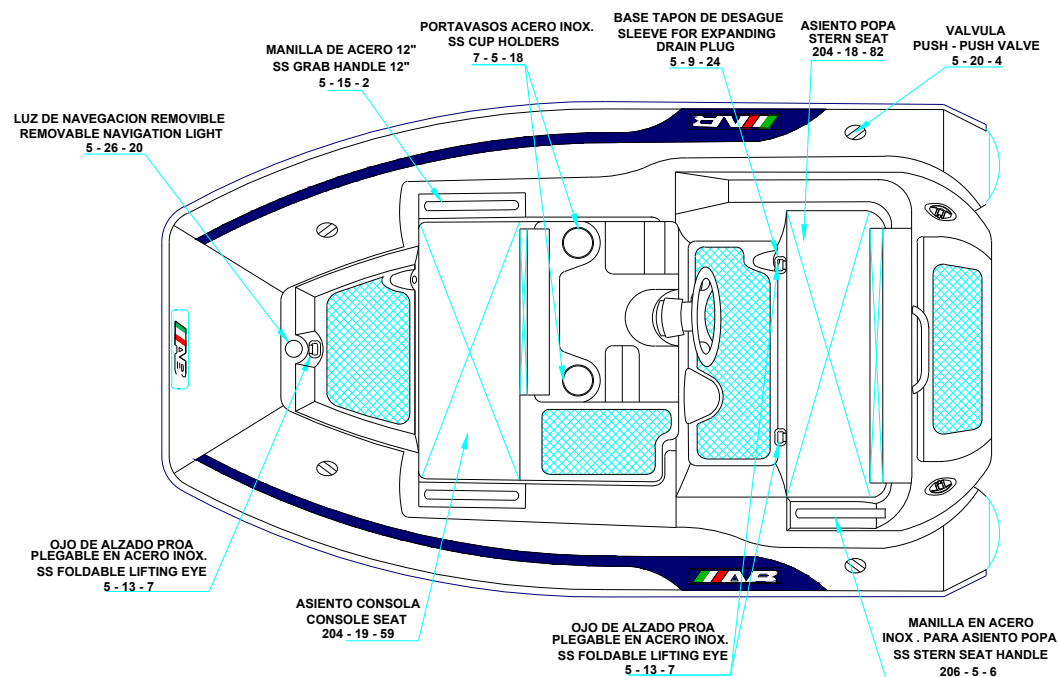
PLANT VIEW VISTA SUPERIOR
