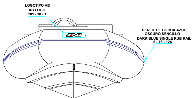
FORE VIEW VISTA FRONTAL
