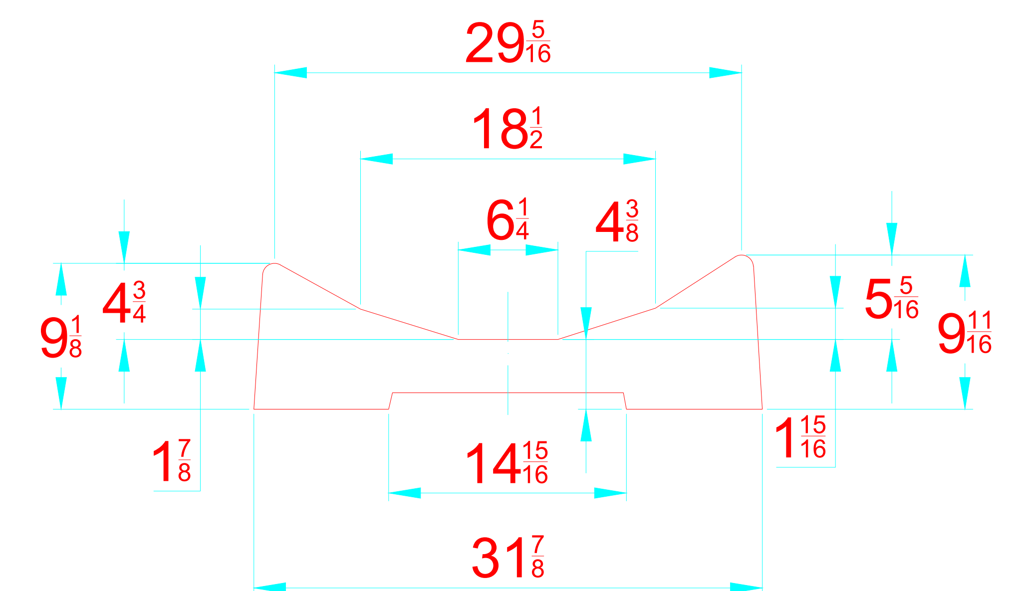
TRANSVERSAL SECTION "A" SECCION TRANSVERSAL "A"
