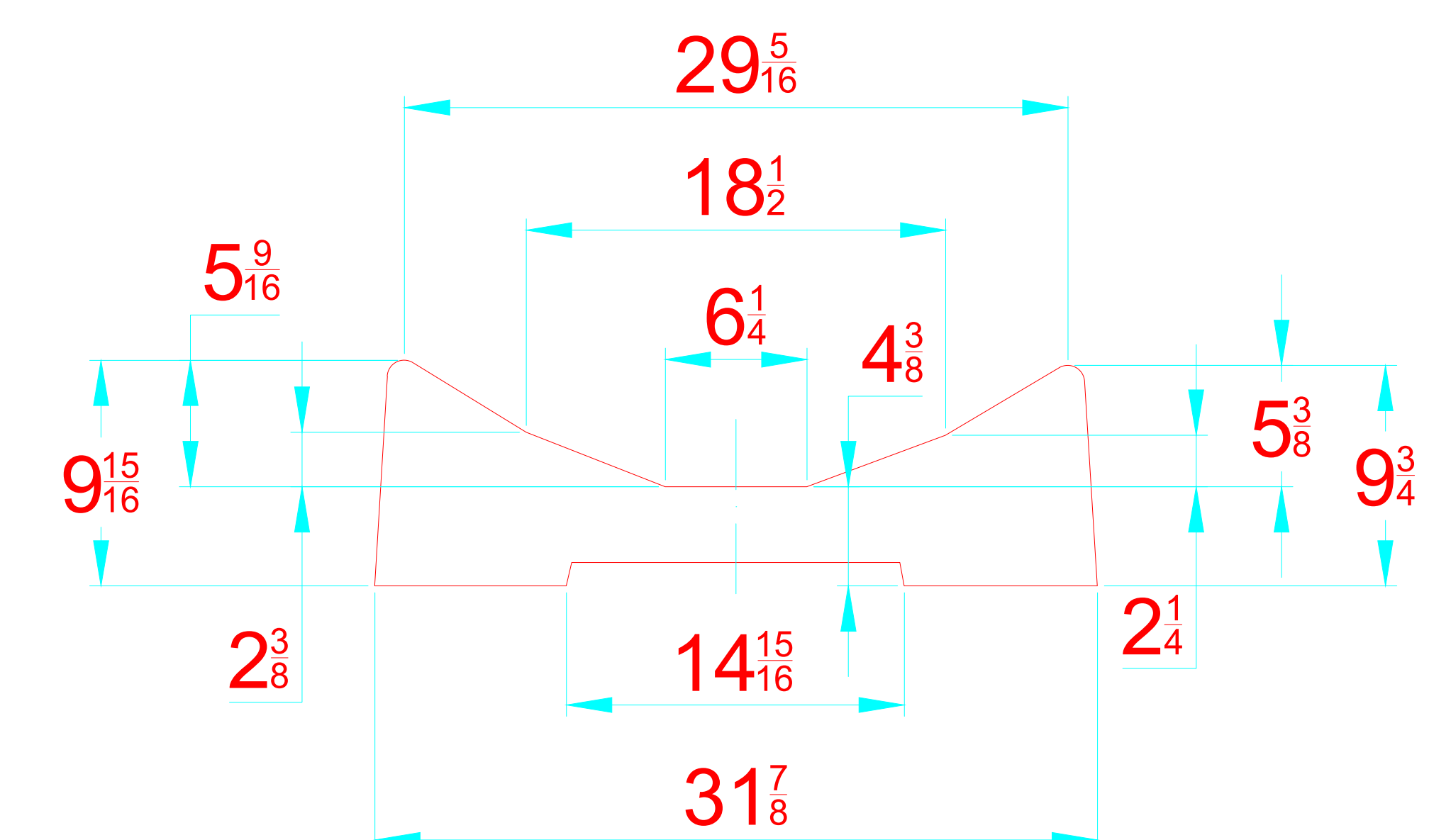
TRANSVERSAL SECTION "A" SECCION TRANSVERSAL "A"
