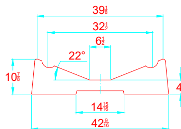
TRANSVERSAL SECTION "A" SECCION TRANSVERSAL "A"
