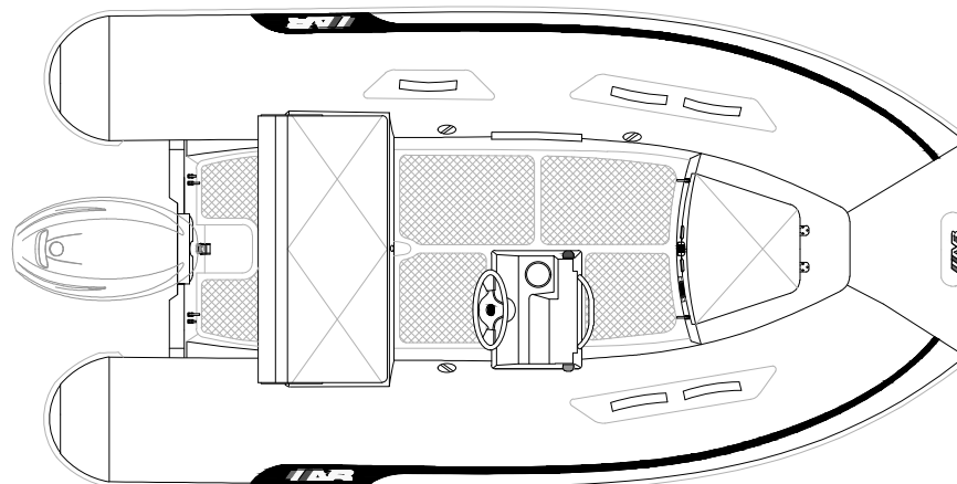
PLANT VIEW
