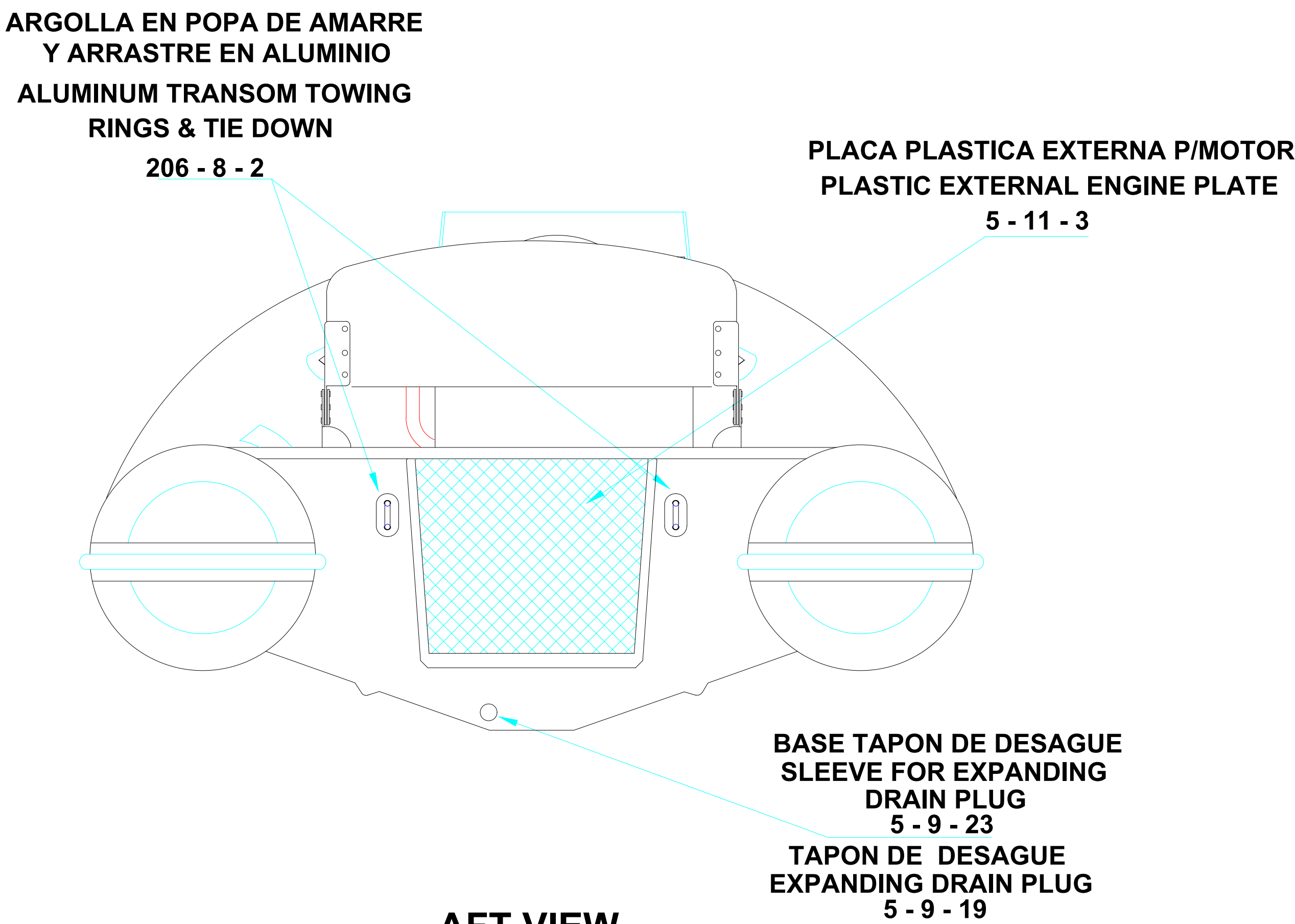
AFT VIEW VISTA TRASERA
