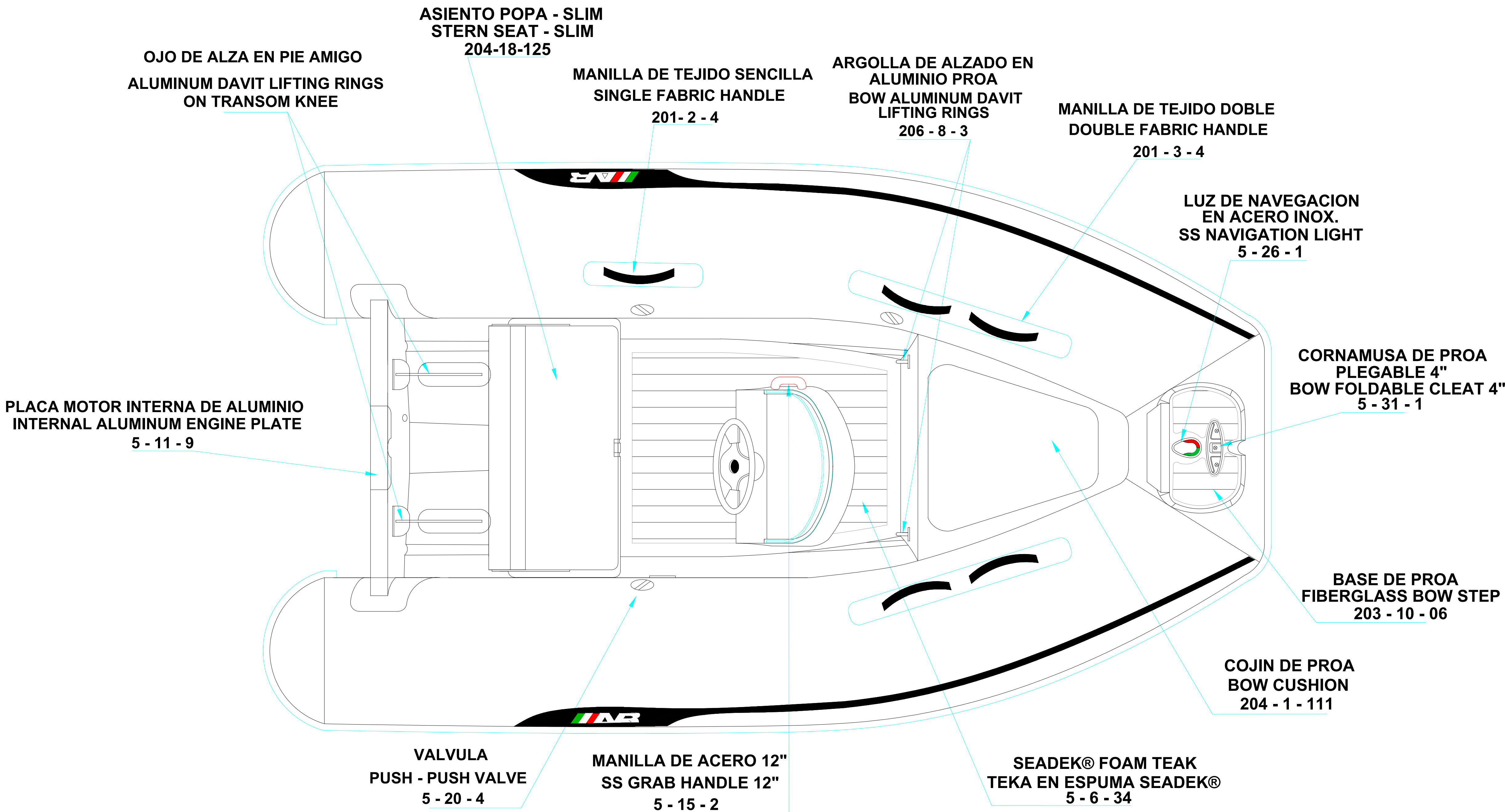
PLANT VIEW VISTA SUPERIOR
