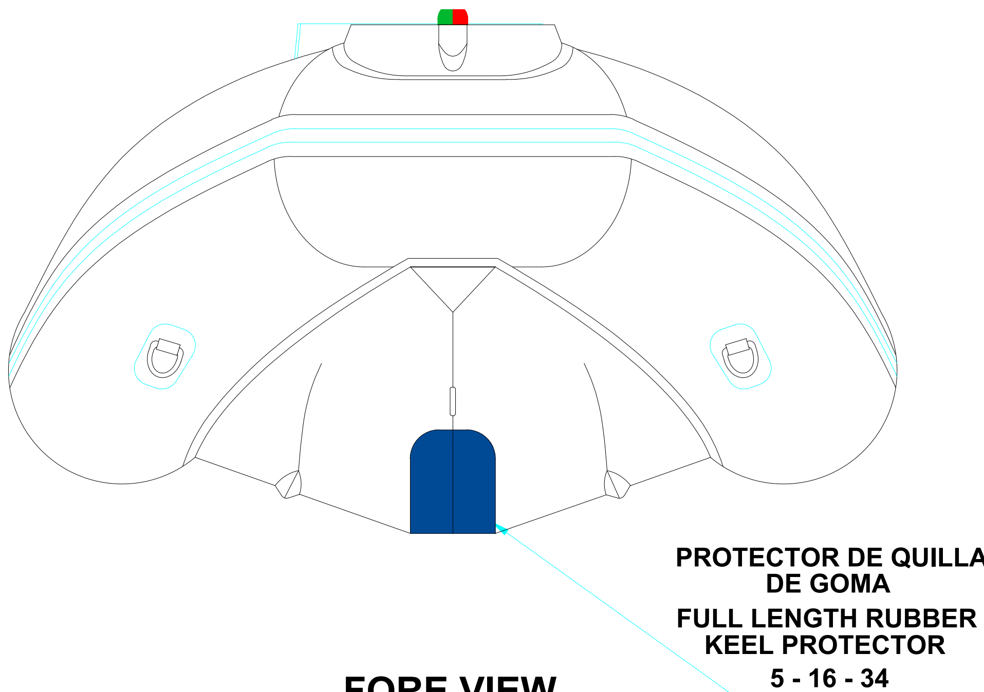
FORE VIEW VISTA FRONTAL
