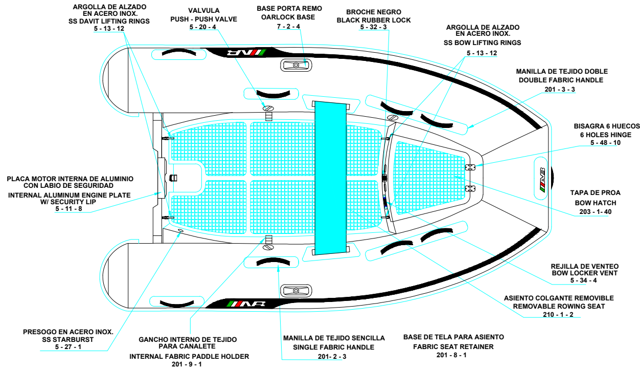
PLANT VIEW VISTA SUPERIOR
