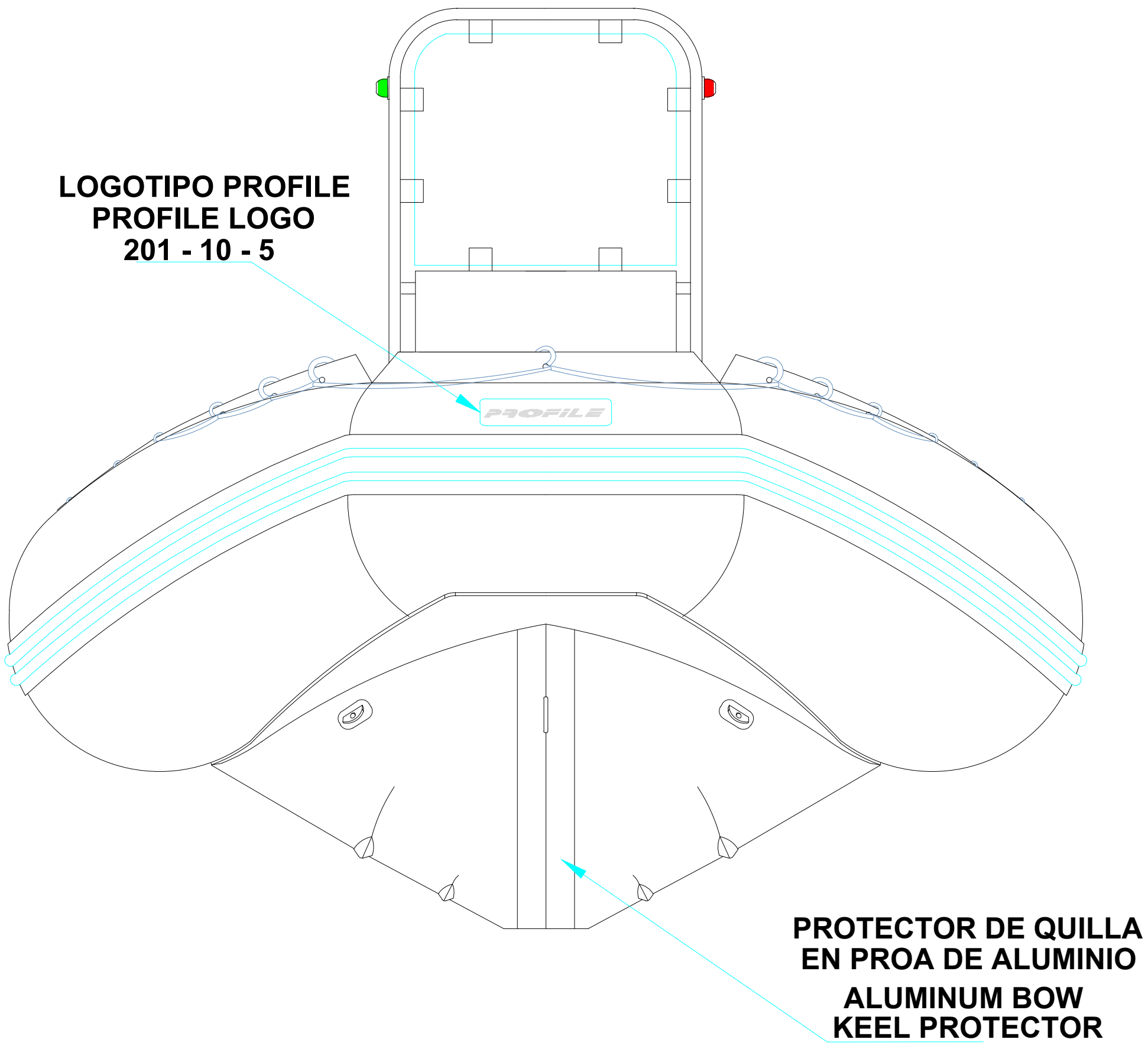
FORE VIEW VISTA FRONTAL
