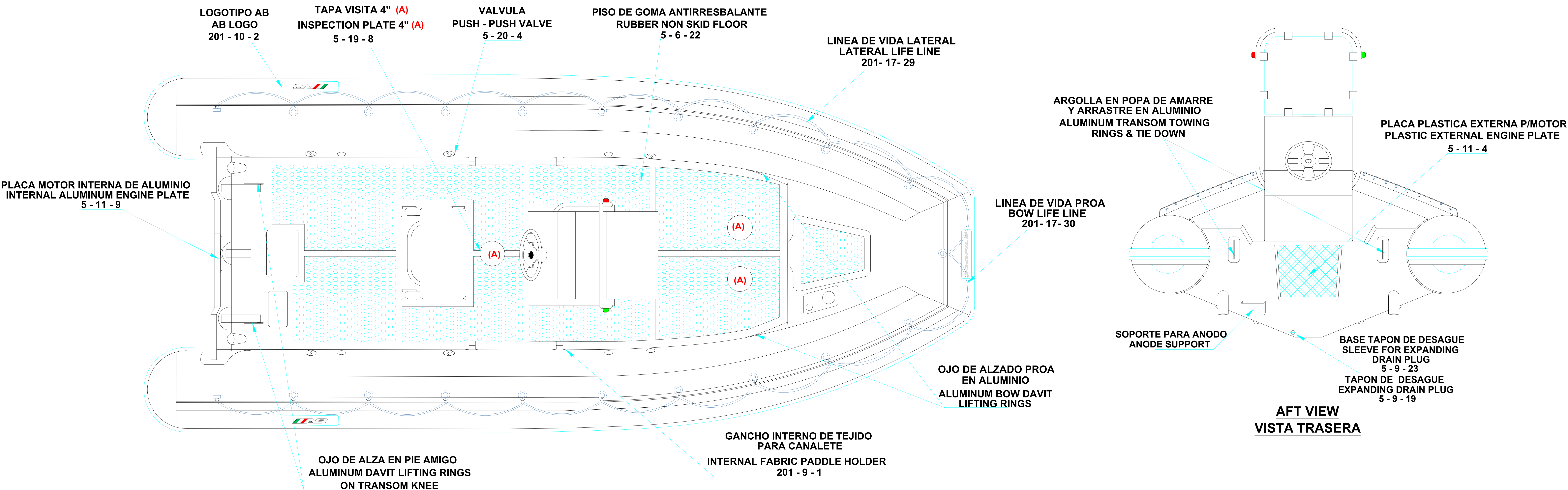
PLANT VIEW VISTA SUPERIOR
