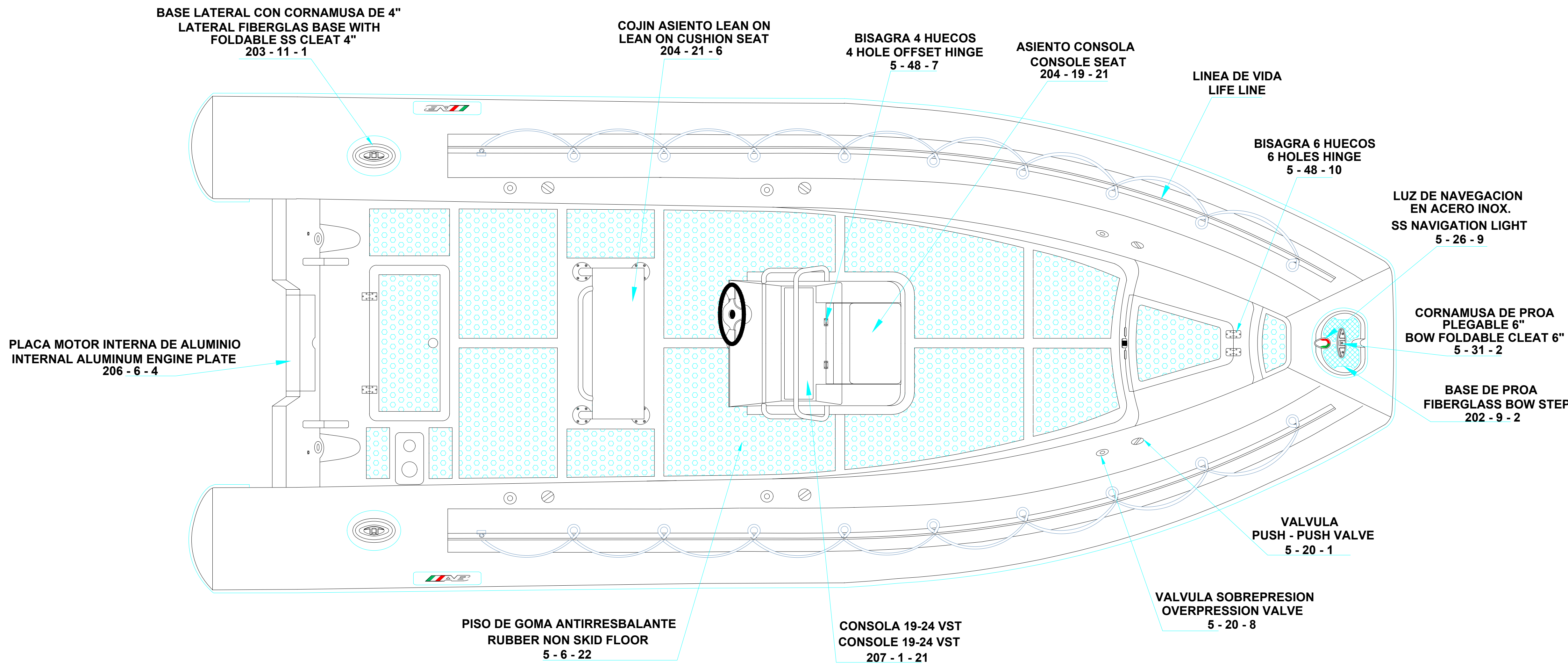
PLANT VIEW VISTA SUPERIOR
