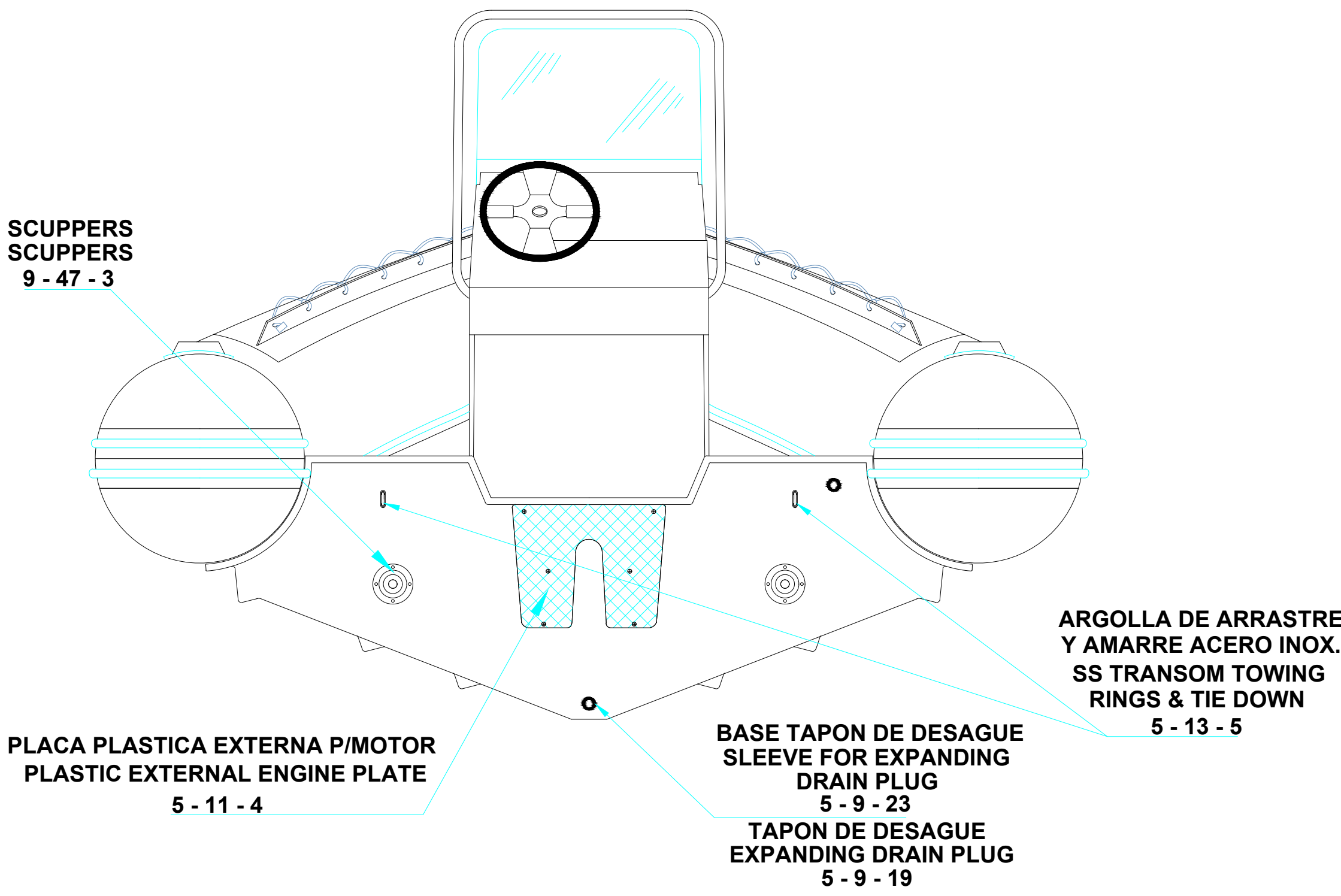
AFT VIEW VISTA TRASERA
