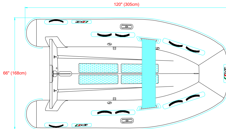
PLANT VIEW VISTA SUPERIOR
