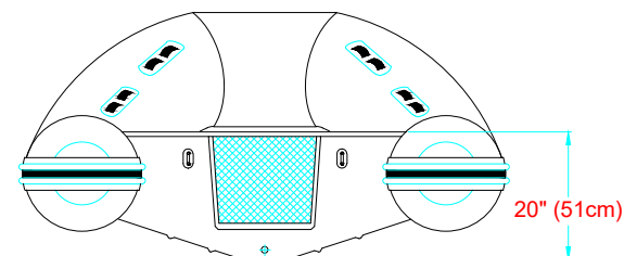
AFT VIEW VISTA TRASERA
