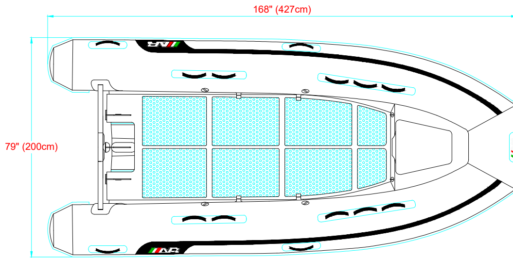
PLANT VIEW VISTA SUPERIOR
