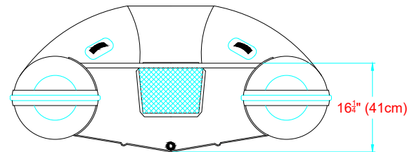
AFT VIEW VISTA TRASERA
