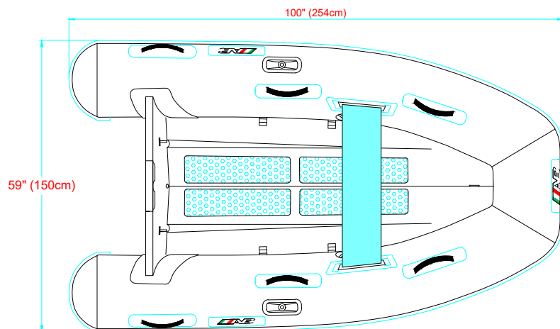
PLANT VIEW VISTA SUPERIOR
