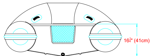
AFT VIEW VISTA TRASERA
