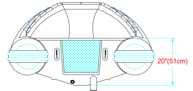
AFT VIEW VISTA TRASERA
