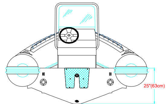
AFT VIEW VISTA TRASERA
