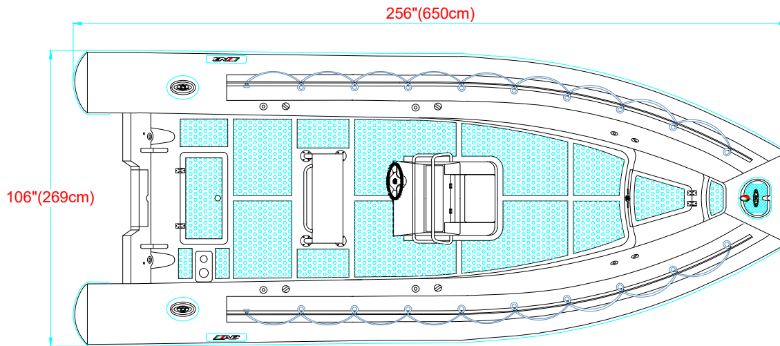
PLANT VIEW VISTA SUPERIOR
