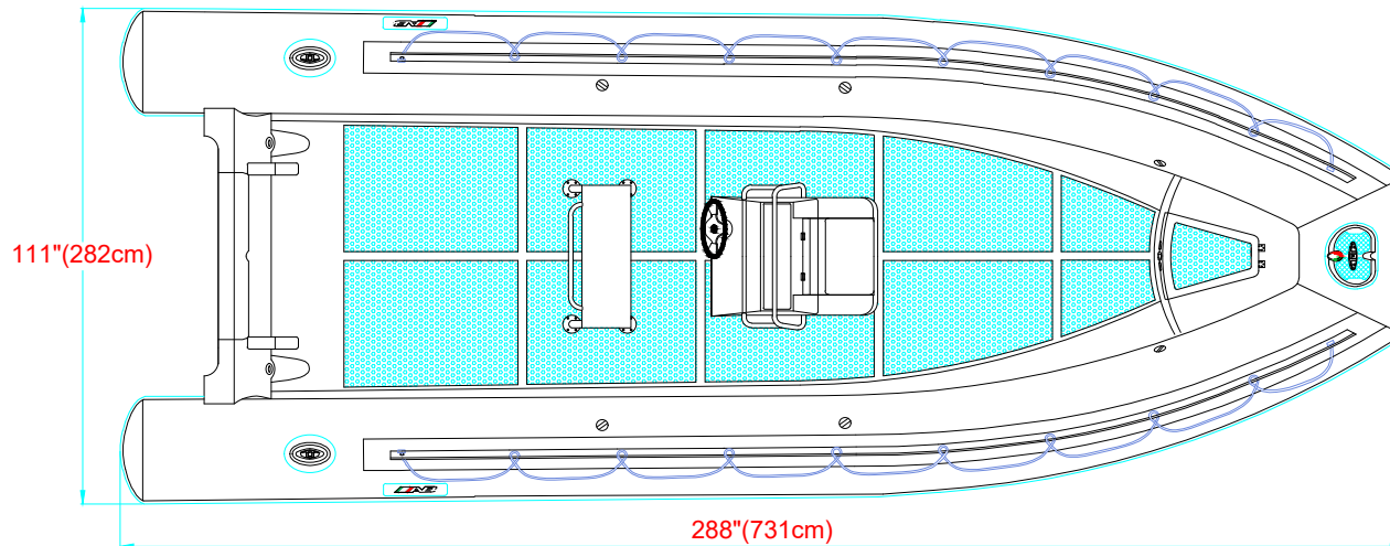
PLANT VIEW VISTA SUPERIOR
