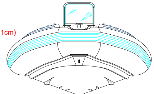
FORE VIEW VISTA FRONTAL
