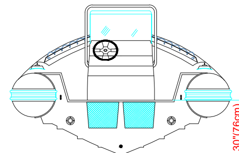
AFT VIEW VISTA TRASERA
